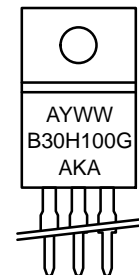
ISOLATED TO-220 CASE 221D STYLE 3
